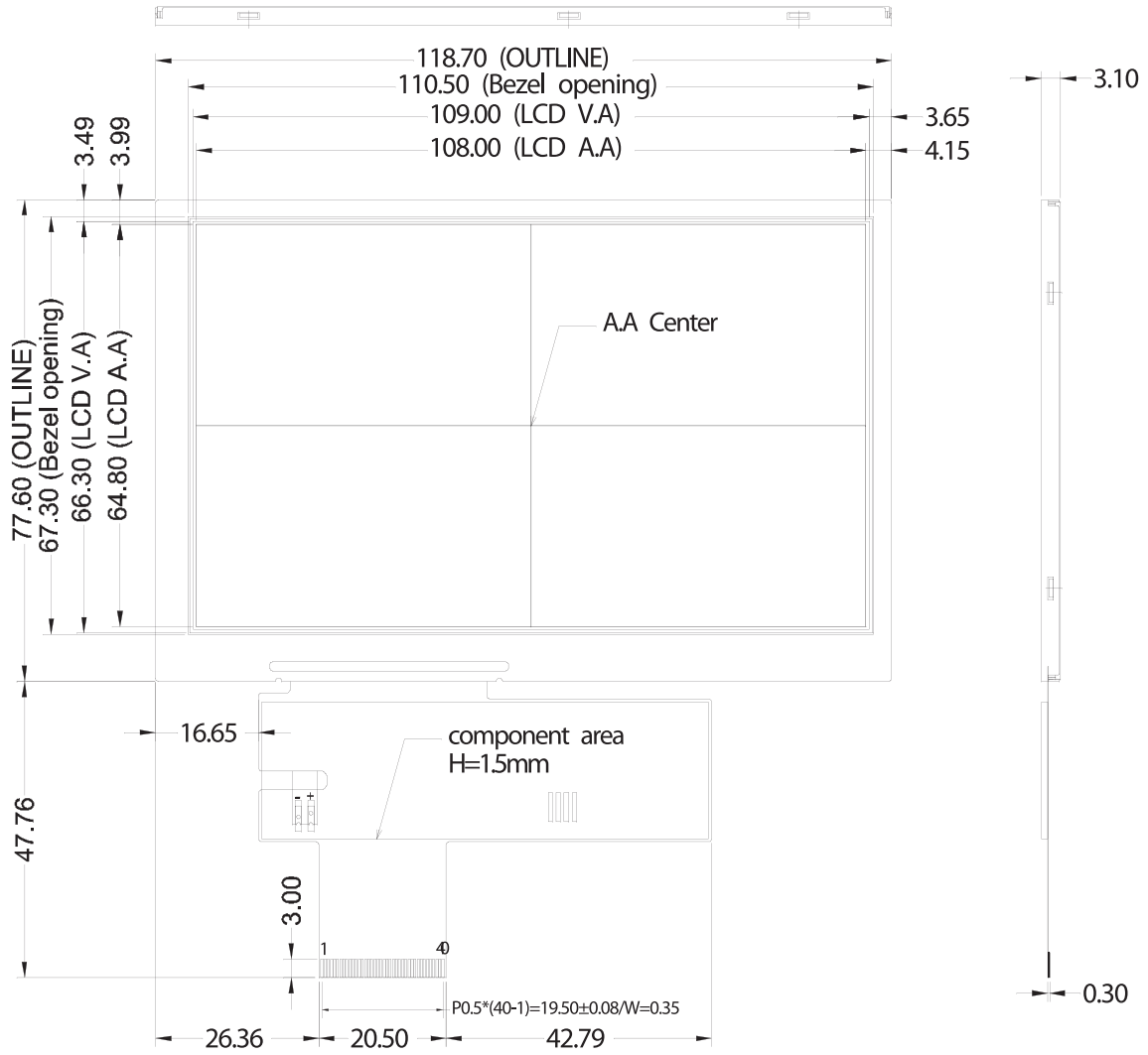
(FH19SC-40S-0.5SH (HIROSE), 40pin, pitch = 0.5mm)
