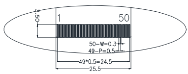
DETAIL A(3:1)
