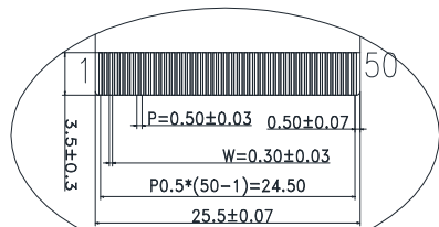
DETAIL A(5:1)
