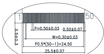
DETAIL A(5:1)
